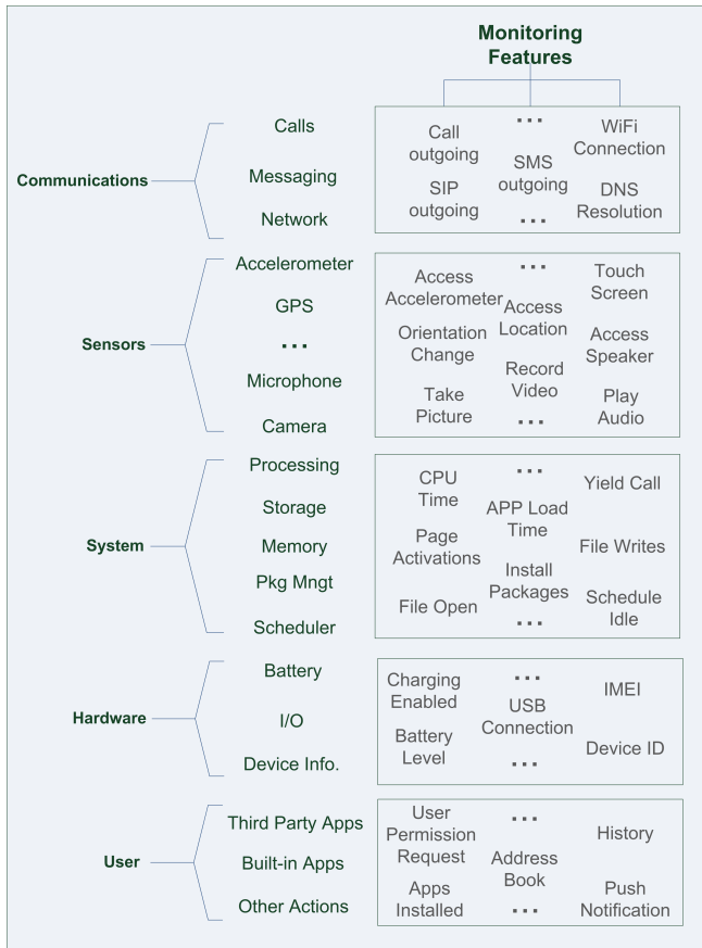
Fig. 6. Taxonomy of monitorable features for smart devices.
